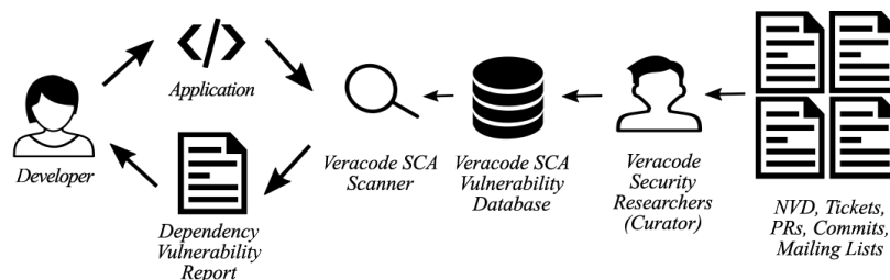
Fig. 2 Overview of Veracode SCA workflow
